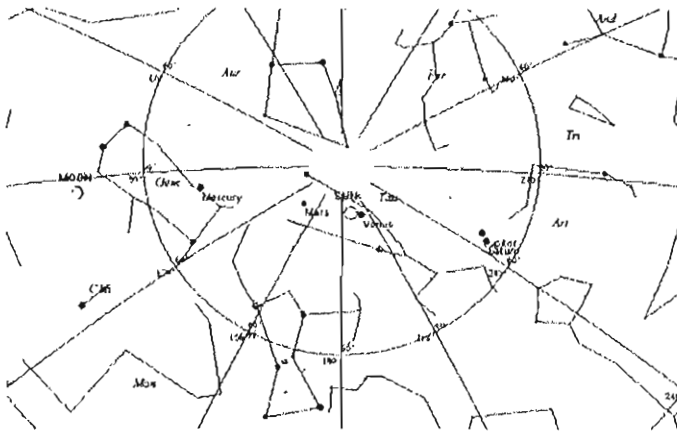
Fig 4: The overhead sky at the time of the event, the Sun is denoted by the circle Chart by SkyMap software
